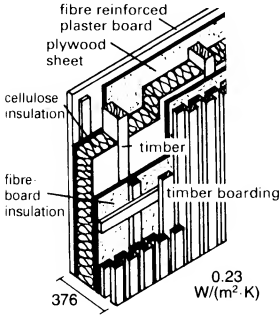
⑦ Low energy wall (Heckmann Ecohouse) 0.23 W/(m 2 ·K)
